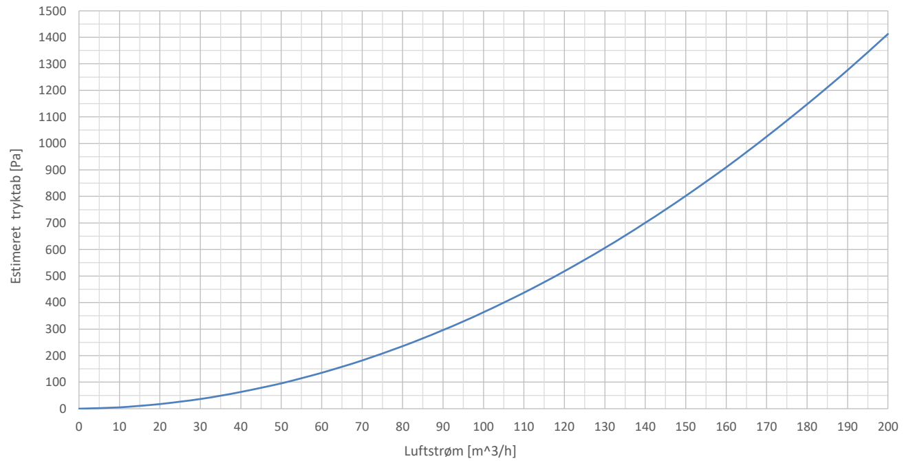
Permavent 11/9 2015, 0 stk ligeud + 2 stk 45 grader + 1 stk 90 grader + 0 stk 135 grader + 0 stk 165 grader + 1,2 meter 57mm kanal
